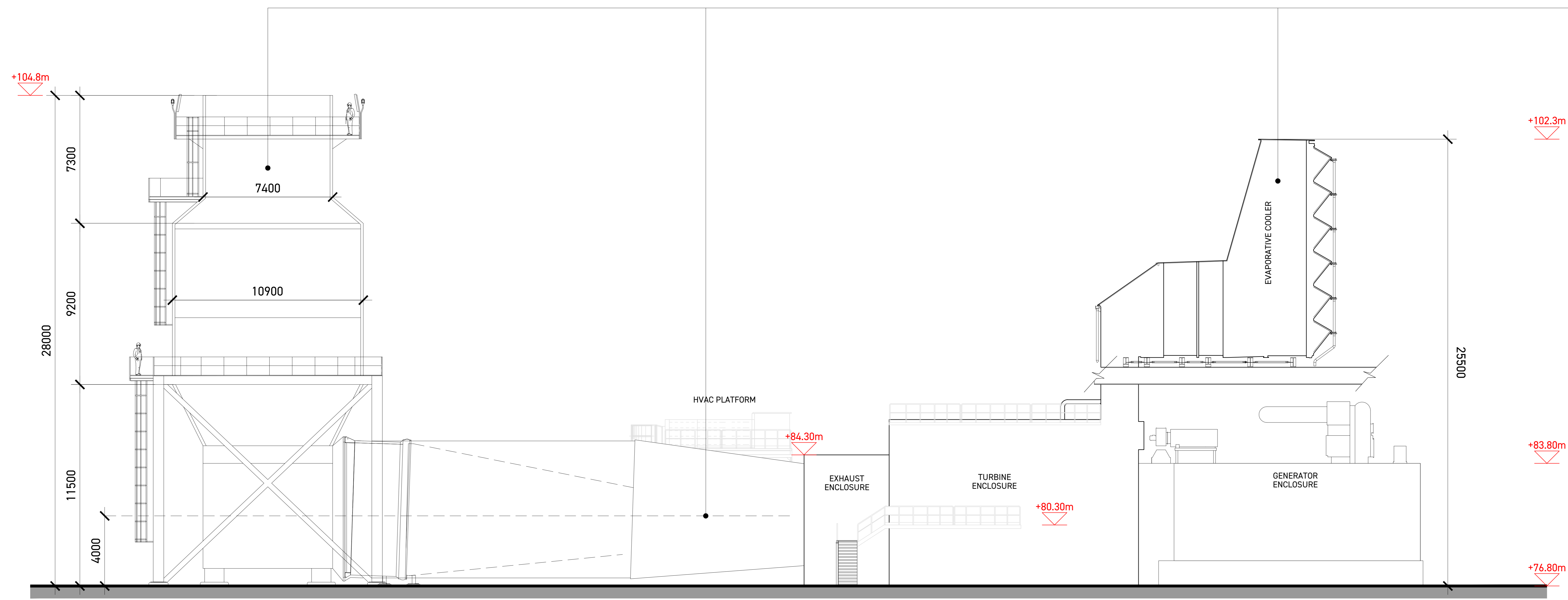
ELEVATION B TO NORTH
